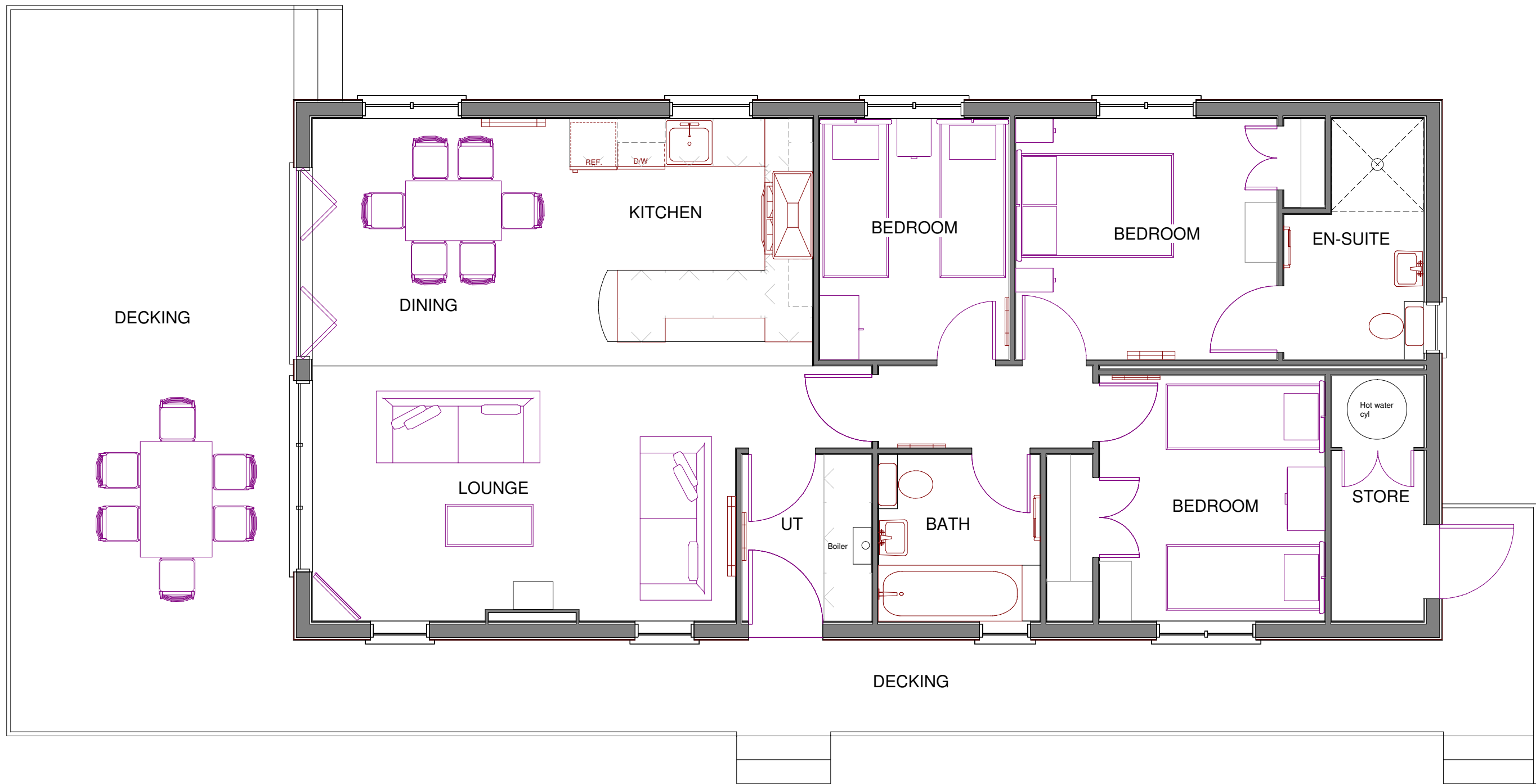
MELVILLE 47 x 22 THREE BED ECO LODGE - LAYOUT PLAN
